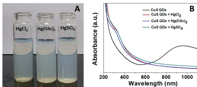
Fig. 7 (A) The colorimetric detection performance and (B) UV-Vis spectra of the CuS QDs in the presence of \text{HgCl}_2 , \text{Hg}(\text{OAc})_2 and \text{HgSO}_4 .
