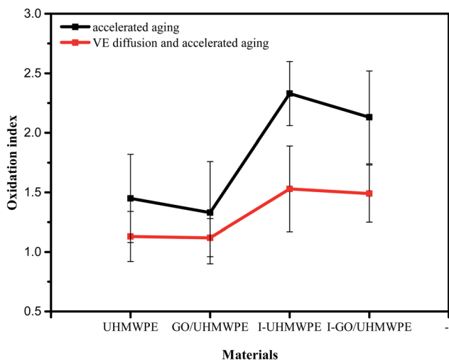
Fig. 15 OI values of different materials.
