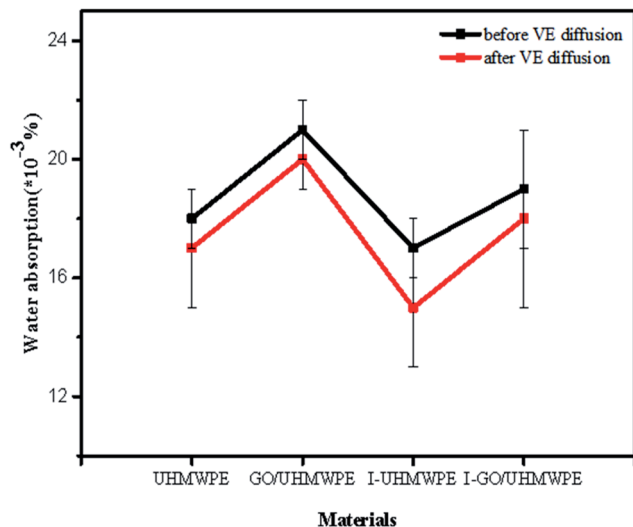
Fig. 12 The water absorption properties of different materials.
