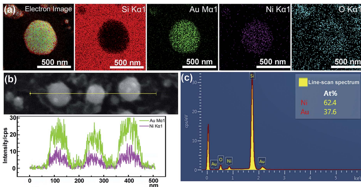
Fig. 3 (a) EDS mapping images of an individual Ni 50 Au 50 nanoparticle and the corresponding element mapping images of Si-K, Au-M, Ni-K and O-K. (b) EDS line-scan analysis of the nanoparticles below 100 nm showing the distribution of the two metals. (c) EDS point-scan spectrum of the particles in (b).
