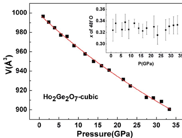
Fig. 7 Observed P – V variation fitted with the third-order Birch–Murnaghan (B–M) equation of state for the cubic \text{Ho}_2\text{Ge}_2\text{O}_7 . The inset shows the pressure dependence of the x parameter for the \text{O}_{48f} atom.
