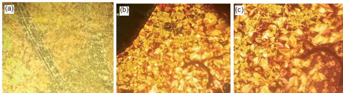
Fig. 3 PLM textures of: (a) the nematic phase of I12_b at 240.0\text{ }^\circ\text{C} upon cooling; (b) smectic A phase of I16_d at 299.0\text{ }^\circ\text{C} upon heating; (c) smectic A phase of I16_d at 280.0\text{ }^\circ\text{C} upon cooling.
