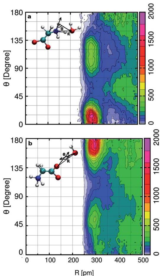
Fig. 2 In the top panel (a) the x-axis represents N–O W distance (in pm), and the y-axis represents the hydrogen bond cut-off angle between two bond vectors N–D N and D N –O W . The bottom panel (b) represents the CDF of O C –O W distance and the hydrogen bond angle that originates from O W –D W and O C –D W bond vectors.
