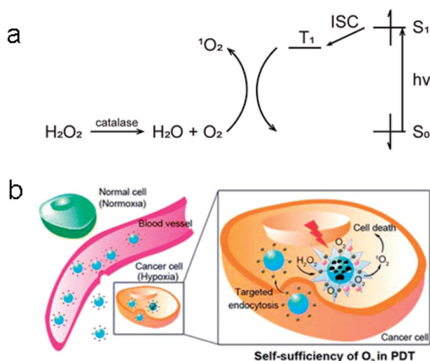
Fig. 3 (a) Catalysis of \text{H}_2\text{O}_2 to \text{O}_2 with catalase and conversion of \text{O}_2 to ^1\text{O}_2 by MB ( \text{S}_0 : singlet ground state; \text{S}_1 : lowest singlet excited state; \text{T}_1 : lowest triplet excited state; ISC: intersystem crossing). (b) The function mechanism of the synthesized nanoparticles. These figures have been adapted from ref. 25 with permission from American Chemical Society.
