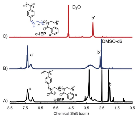
Fig. 1 ^1\text{H} NMR spectra of (A) c-iMP, (B) c-iEP in DMSO- d_6 and (C) c-iEP in hot \text{D}_2\text{O} ( 70^\circ\text{C} ).
