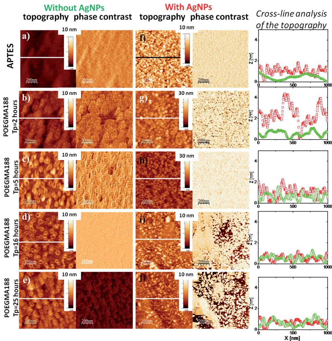
Fig. 2 Representative AFM images (topography and phase contrast, recorded in a dry state) of the glass surface silanized with APTES (a) and subsequently functionalized with grafted POEGMA188 brushes (b–e, using different polymerization times T_p ), compared with the data for the same substrates incorporating AgNPs (f–j) after a 15 min long exposure to 5 mM \text{AgNO}_3 solution, followed by reduction in 0.2 M \text{NaBH}_4 solution for 12 h. Cross-line analysis corresponds to the topography of the samples without (green) and with AgNPs (red).
