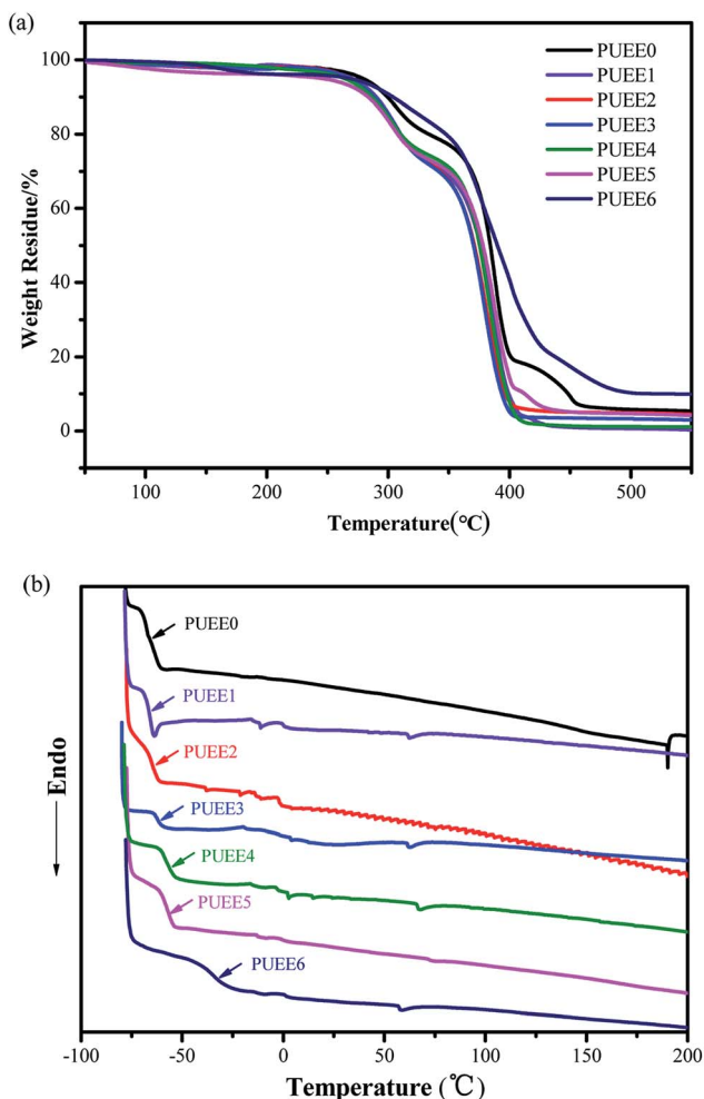
Fig. 4 (a) TGA and (b) DSC curves of the PUEEs in a nitrogen atmosphere at the heating rates of 10 °C min -1 and 5 °C min -1 , respectively.
