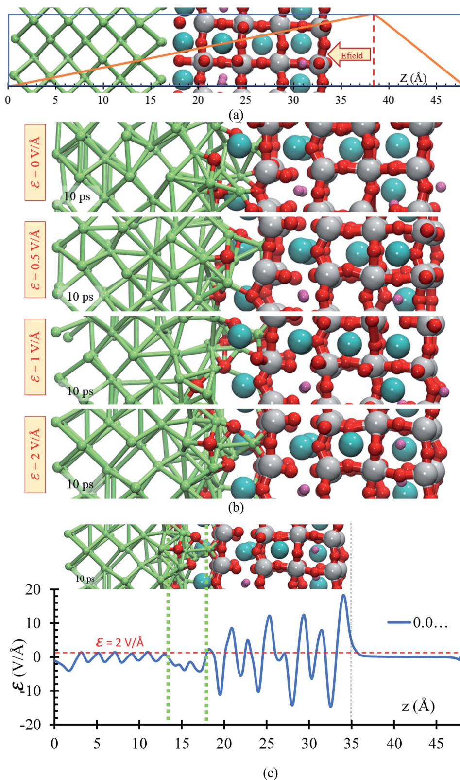
Fig. 6 (a) \text{Li}_{0.29}\text{La}_{0.57}\text{TiO}_3/\text{Li} -metal electrochemical cell under the application of an external electric field. (b) Structural changes of the \text{Li}_{0.29}\text{La}_{0.57}\text{TiO}_3/\text{Li} -metal interface at 10 ps of applying external electric fields of \epsilon = 0, 0.5, 1 and 2 \text{ V \AA}^{-1} . (c) Profile average of the internal electric field component in the drift direction of transport of ions. (d) Atomic profile along the z axis at different time rates, for the four cases, \epsilon = 0, 0.5, 1, 2 \text{ V \AA}^{-1} .
