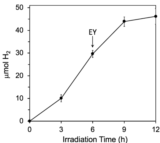
Fig. 7 Effect of adding more EY during photosensitized H_2 generation conditions are the same as listed in the Fig. 6 legend, except that an additional 72 \mu M more EY was added at 6 h, as indicated by the arrow.
