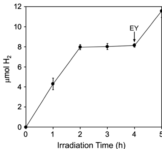
Fig. 8 Photosensitized H_2 production upon white light irradiation of an aerobic Pt/Fe-Hfn solution of composition identical to that listed in the Fig. 6 legend. The arrow indicates addition of 72 \mu M more EY. ‡
