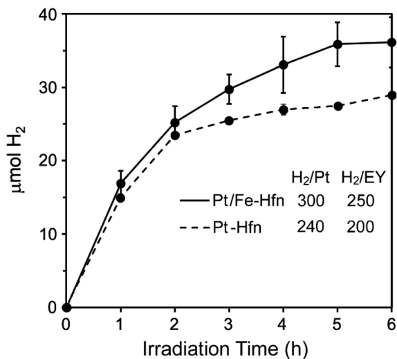
Fig. 6 Time courses for photosensitized H_2 production from a solution of either Pt-Hfn or Pt/Fe-Hfn at 60 \mu M Pt and 72 \mu M EY in 0.3 M TEOA pH 9 upon white light irradiation. ‡ H_2/Pt and H_2/EY values represent 6 h TONs (mol H_2 /mol Pt or mol EY).
