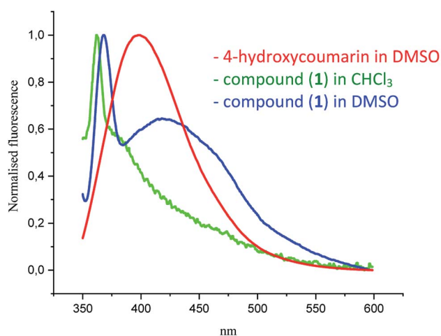
Fig. 4 Normalized fluorescence spectra of compound ( 1 ) in DMSO and chloroform ( 2.64 \times 10^{-6} M, \lambda_{\text{exc}} = 320 nm) and 4-hydroxycoumarin ( 7.03 \times 10^{-7} M, \lambda_{\text{exc}} = 320 nm) in DMSO.
