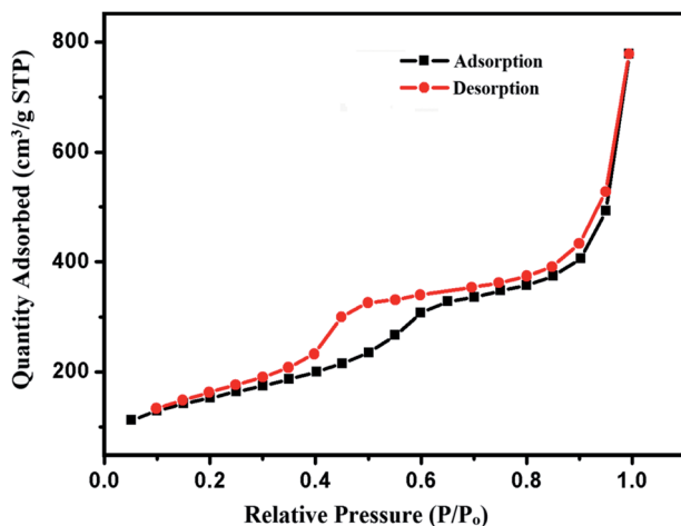
Fig. 8 \text{N}_2 adsorption–desorption isotherm of c\text{SiO}_2@DFNS .
