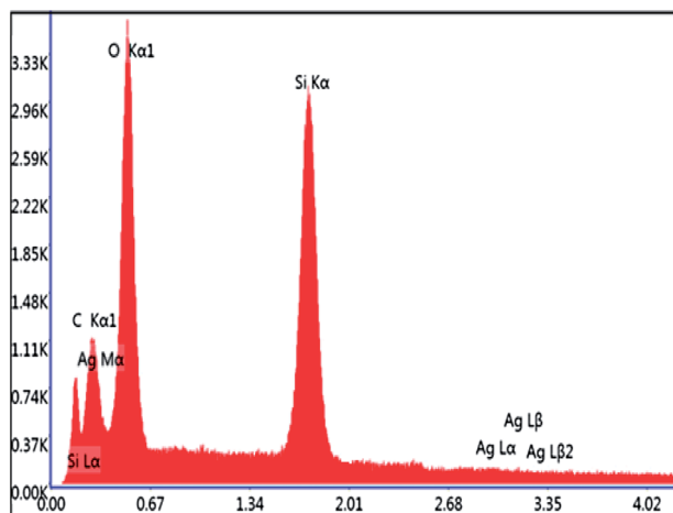
Fig. 7 EDS spectrum of c\text{SiO}_2@DFNS@Ag .
