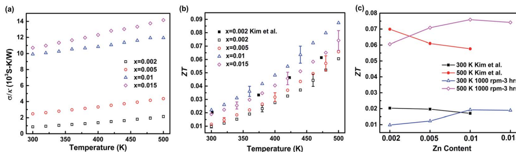
Fig. 6 (a) Ratio of electrical conductivity to thermal conductivity and (b) ZT of the hot-pressed \text{Ga}_{1-x}\text{Zn}_x\text{Sb} nanocomposites with different amounts of Zn doping ( x = 0.002, 0.005, 0.01 , and 0.015 ); (c) variation of the ZT with the Zn content at 300 K and 500 K. The uncertainty in ZT is within 11%. The results reported by Kim et al. 20 for the bulk alloy are also shown in (b) and (c) for comparison.
