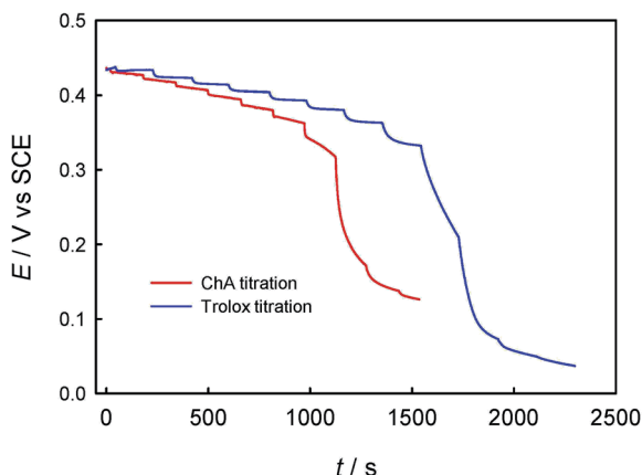
Fig. 2 Potentiometric titration curve on GCE for the successive additions of ChA (addition of 5\text{ }\mu\text{L} of 0.500\text{ mM} ChA for each) into 4.0\text{ mL} of 0.1\text{ M} phosphate buffer (pH 7.4) containing 0.1\text{ M} Na_2SO_4 , 40\text{ }\mu\text{M} ABTS and 47.5\text{ }\mu\text{M} ABTS^{*+} , or of trolox (addition of 10\text{ }\mu\text{L} of 1.00\text{ mM} trolox for each) into 4.0\text{ mL} of 0.1\text{ M} phosphate buffer (pH 7.4) containing 0.1\text{ M} Na_2SO_4 , 43.7\text{ }\mu\text{M} ABTS and 43.8\text{ }\mu\text{M} ABTS^{*+} .
