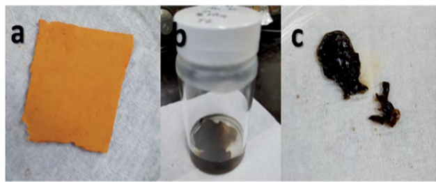
Fig. 3 Electrospun nanofiber samples (a) before sulfonation, (b) during sulfonation with concentrated sulfuric acid at 72 h, and (c) after washing, which formed into a gel.
