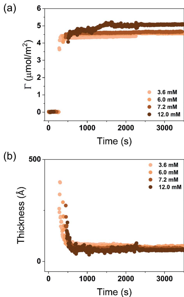
Fig. 6 (a) Time evolution of the adsorbed amount, \Gamma , and (b) average layer thickness, d , of DODAC–water–butyric acid mixtures at the silica/water interface ( T = 25 °C). Mixtures with increasing concentration in the ellipsometry cuvette, 3.6 mM (C1), 6.0 mM (C2), 7.2 mM (C3) and 12.0 mM (C4).
