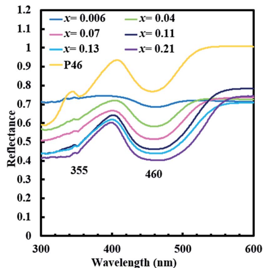
Fig. 9 Diffuse reflectance spectra of (Y_{1-x}Ce_x)_3Al_5O_{12} crystals.
