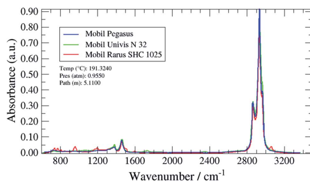
Fig. 10 Overlaid target oil sample spectra.
