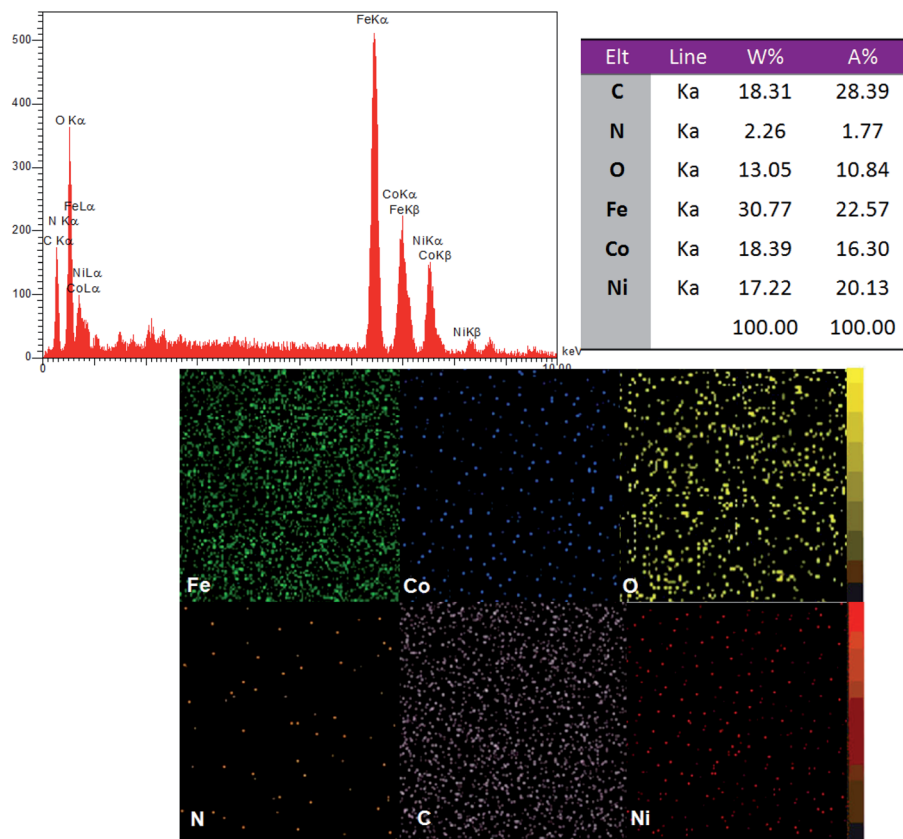
Fig. 4 EDX spectrum and elemental mapping of \text{CoFe}_2\text{O}_4@GO-K 22 \cdot Ni nanocomposite.
