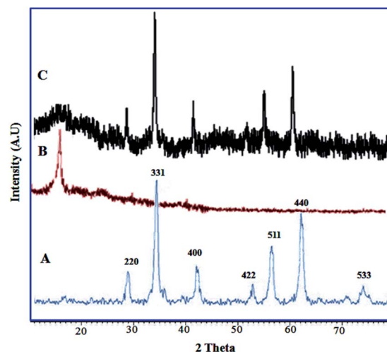
Fig. 5 XRD patterns of \text{CoFe}_2\text{O}_4 (A), GO (B) and \text{CoFe}_2\text{O}_4@GO-K 22 \cdot Ni (C).
