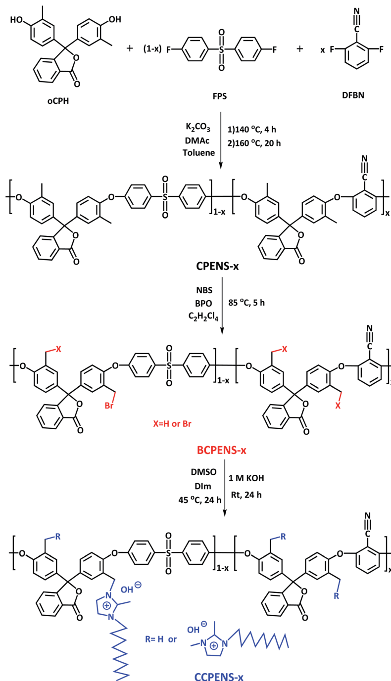
Scheme 1 Synthesis of CPENS- x , BCPENS- x and CCPENS- x .
