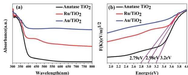
Fig. 10 UV-Vis absorbance spectra (a) and Kubelka-Munk plots of anatase \text{TiO}_2 , \text{Ru}/\text{TiO}_2 , and \text{Au}/\text{TiO}_2 photocatalysts (b), respectively.
