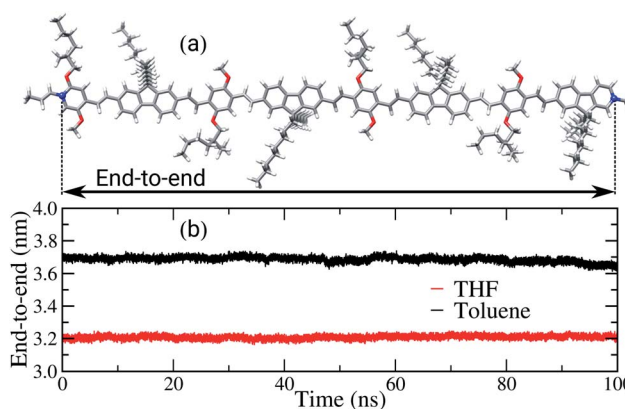
Fig. 5 (a) Schematic illustration of end-to-end distance, arrows between the blue atoms and (b) time evolution of the PFO-MEH-PPV end-to-end distance, calculated for the film formed from THF (red) and for toluene (black).
