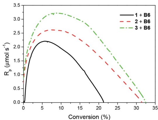
Fig. 4 Rate vs. conversion for photopolymerization of TMPTA initiated by 1/B6, 2/B6 and 3/B6, cured r.t. by visible light (488 nm) with an intensity of 100 \text{ mW cm}^{-2} (The photoinitiator concentration is 0.0075 \text{ M} ).
