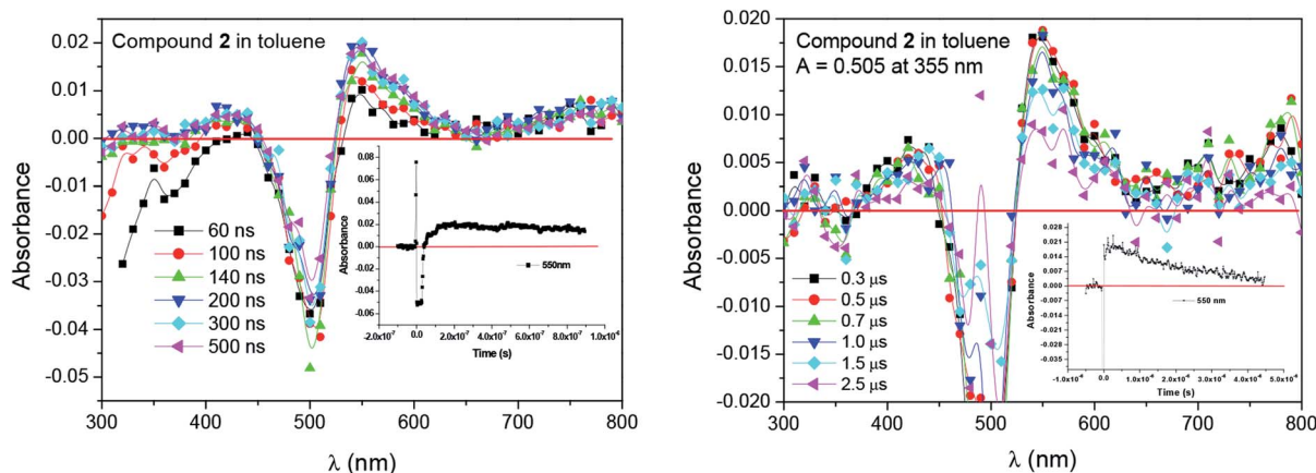
Fig. 5 Laser flash photolysis spectra of the dye 2 in toluene recorded after irradiation with laser pulses of 355 nm. Delay times shown in legends. Inset: kinetic curves for the growth (left) and the decay (right) of absorbance (550 nm) of 2 in toluene.
