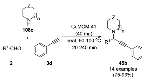
Scheme 70 A 3 coupling catalyzed by CuMCM-41.
