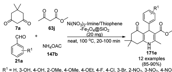
Scheme 273 \text{Ni}(\text{NO}_3)_2 -imine/thiophene- \text{Fe}_3\text{O}_4@SiO_2 NP-catalyzed synthesis of polyhydroquinolines (171e).
