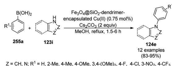
Scheme 258 \text{Fe}_3\text{O}_4@SiO_2\text{-dendrimer-encapsulated Cu(II)} -catalyzed synthesis of benzazoles (124e).
