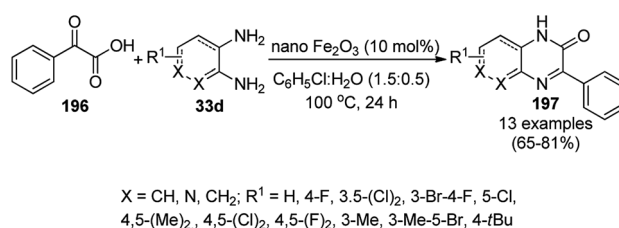
Scheme 105 Reactions of 2-oxo-2-phenylacetic acid ( 197 ) with substituted benzene-1,2-diamines ( 33d ) in the presence of superparamagnetic \text{Fe}_2\text{O}_3 NPs. 216
