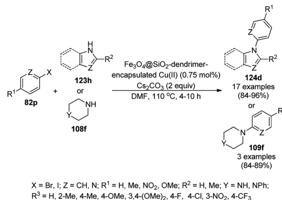
Scheme 257 Synthesis of arylated N -containing heterocycles (124d/109f) using \text{Fe}_3\text{O}_4@SiO_2\text{-dendrimer-encapsulated Cu(II)} catalyst.
