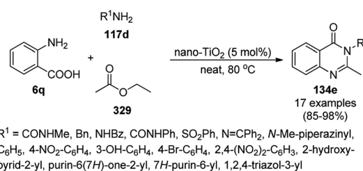
Scheme 226 Nano- \text{TiO}_2 NP-catalyzed three-component reaction of o -amino benzoic acid ( 6q ), ethyl acetate ( 329 ) and amine ( 117d ).
