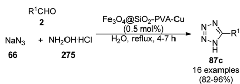
Scheme 256 Synthesis of 5-aryl tetrazoles (87c) catalyzed by \text{Fe}_3\text{O}_4@SiO_2\text{-TCT-PVA-Cu(II)} .
