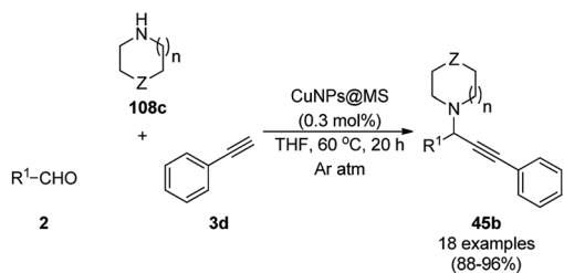
Scheme 68 Synthesis of propargylamines ( 45b ) catalyzed by CuNPs@MS.
