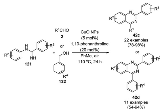
Scheme 47 CuO NP-catalyzed synthesis of quinazolines (41c/d).
