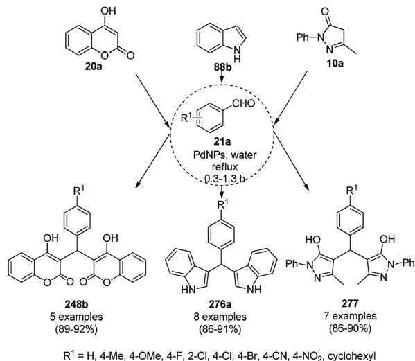
Scheme 167 Green synthesis of bis(heterocyclil)methanes in water catalyzed by PdNPs.
