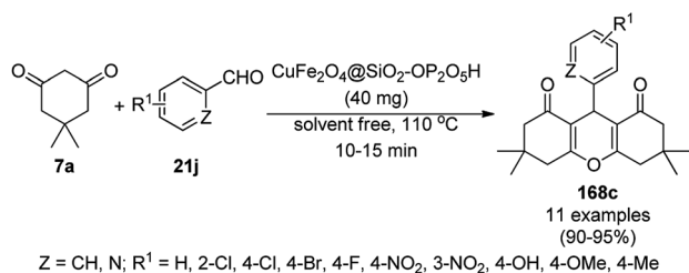
Scheme 240 Synthesis of 1,8-dioxo-octahydroxanthenes ( 168c ) using \text{CuFe}_2\text{O}_4@SiO_2-OP_2O_5H MNP catalyst.
