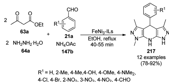
Scheme 116 \text{FeNi}_3 -ILs catalyzed synthesis of the tetrahydrodipyrazolo pyridines ( 217 ).
