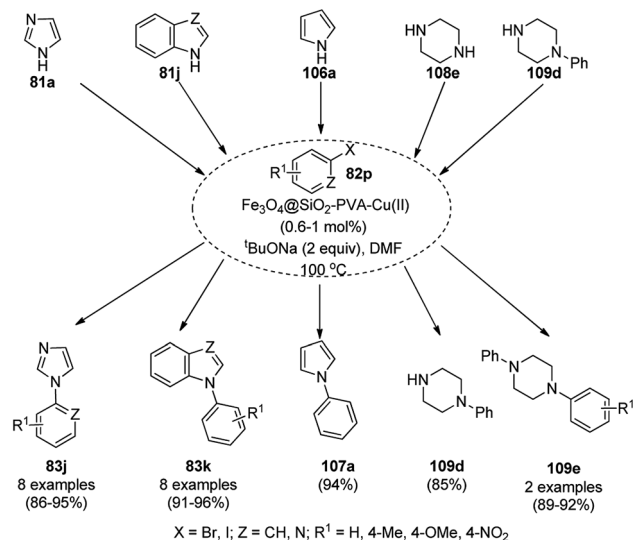
Scheme 255 Synthesis of N -arylated heterocycles catalyzed by \text{Fe}_3\text{O}_4@SiO_2\text{-TCT-PVA-Cu(II)} .
