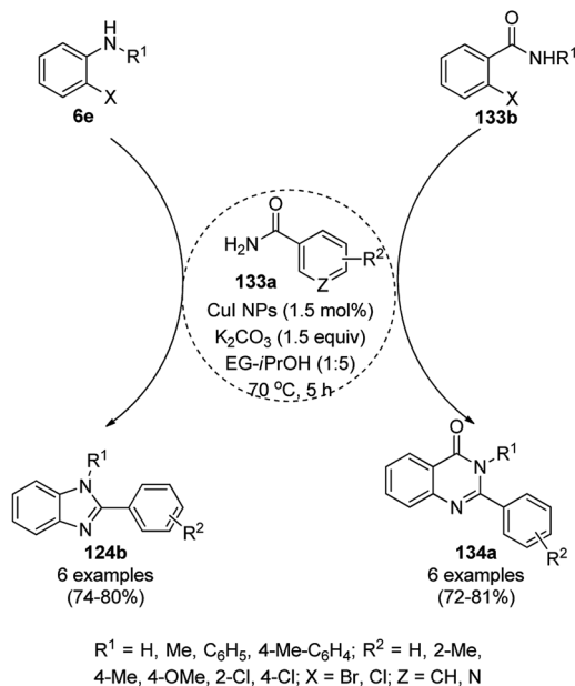
Scheme 53 CuI NP-catalyzed synthesis of benzimidazoles ( 124b ) and quinazolines ( 134a ).
