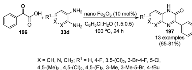
Scheme 105 Reactions of 2-oxo-2-phenylacetic acid ( 196 ) with substituted benzene-1,2-diamines ( 33d ) in the presence of superparamagnetic Fe 2 O 3 NPs. 216
