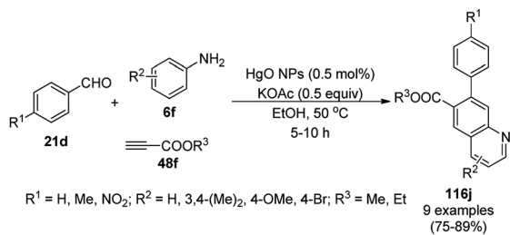
Scheme 235 Synthesis of quinolines ( 116j ) catalyzed by tetraphenylcyclopentandienone@HgO NPs.
