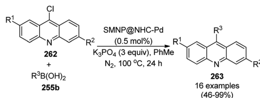
R 1 = H, Cl; R 2 = H, OMe; R 3 = cyclopropyl, 2-phenethyl-1-yl, 2-phenethenyl-1-yl; C 6 H 5 , 2-Me-C 6 H 4 , 3-Me-C 6 H 4 , 4-Me-C 6 H 4 , 4- t Bu-C 6 H 4 , 3,4-(Me) 2 -C 6 H 3 , 2-OMe-C 6 H 4 , 4-OMe-C 6 H 4 , 2-SMe-C 6 H 4 , 4-SMe-C 6 H 4 , 4-F-C 6 H 4 , 4-Cl-C 6 H 4 , 2,4-(F) 2 -C 6 H 3 , 4-CF 3 -C 6 H 4 , 1-naphthyl, 2-naphthyl, 2-furyl
