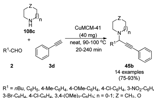
Scheme 70 \text{A}^3 coupling catalyzed by \text{CuMCM-41} .
