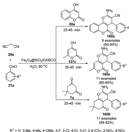
Scheme 101 Synthesis of 4 H -benzo[ b ]pyran derivatives ( 160a/e/b ) catalyzed by \text{Fe}_3\text{O}_4@(\text{SiO}_2)_n /DABCO.
