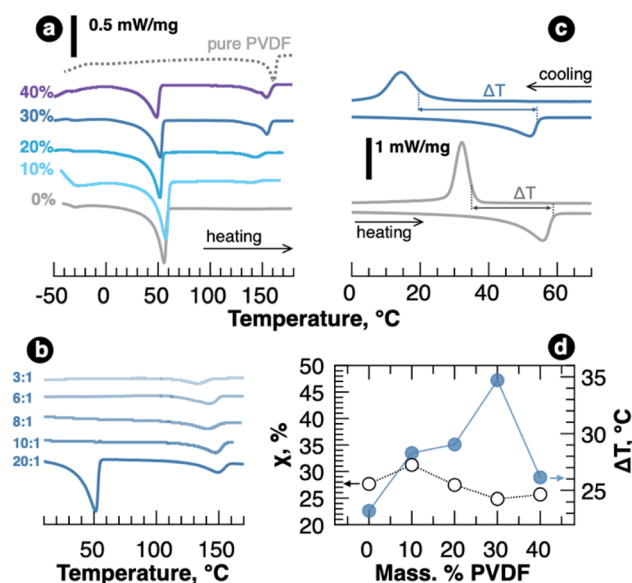
Fig. 3 DSC curves for polymer films with EO : Li ratio of 20 : 1 and various PVDF content (a) and for the samples with 30 wt% PVDF and various EO : Li ratio (b). The data were recorded at 10 °C min -1 heating rate. (c) Heating and cooling DSC curves (10 °C min -1 rate) for the samples with 0 and 30 wt% PVDF and LiTFSI concentration corresponding to EO : Li of 20 : 1. (d) Dependence of PEO crystallinity ( \chi ) and the temperature range ( \Delta T ), in which PEO is fully amorphous, on the wt. fraction of PVDF for the films with EO : Li of 20 : 1.
