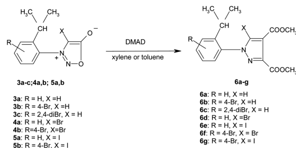
Scheme 3 The synthesis of the halogenated 1-arylpdrazoles 6a-g .
