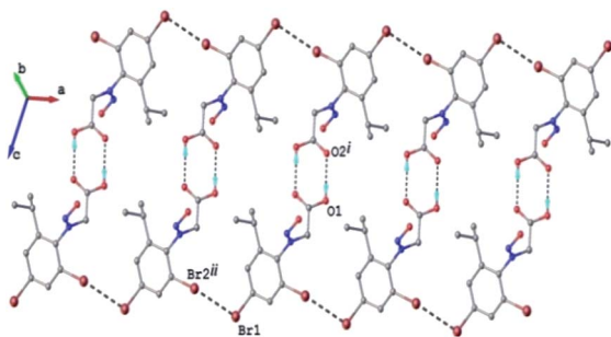
Fig. 3 1D supramolecular network in the crystal structure 2c . H-atoms not involved in hydrogen bonding are omitted. H-bonds and \text{Br}\cdots\text{Br} contacts are shown in dashed-black lines.
