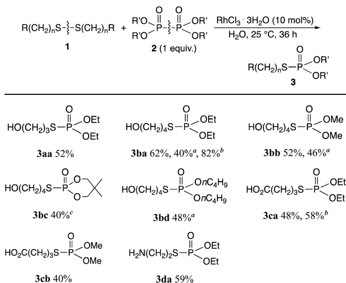
a At 40 °C for 36 h. b Use of \text{RhCl}_3 \cdot 3\text{H}_2\text{O} (20 mol%). c At 70 °C for 36 h.
