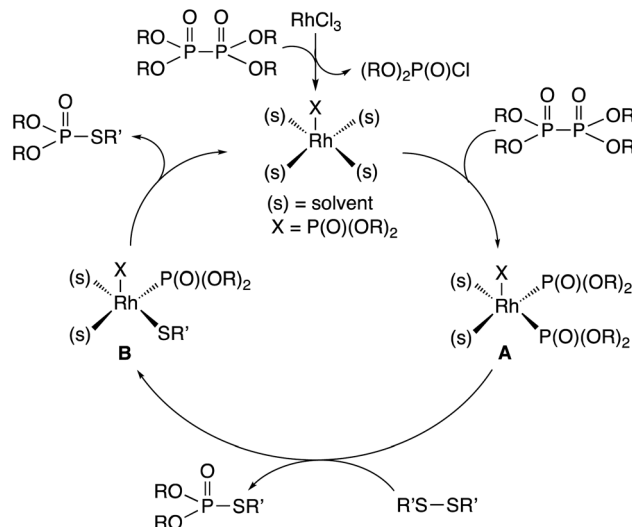
Fig. 1 Proposed reaction mechanism.
