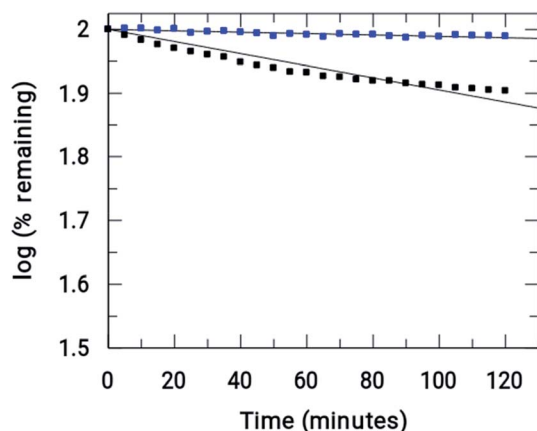
Fig. 7 Comparison of the rate of reductions of Onz (■) and [Zn(Onz) 2 Cl 2 ] (■) under anaerobic conditions. (initial concentrations = 0.2 U mL -1 in XOD, 80 μM in Onz or Zn(Onz) 2 Cl 2 in the mixture, 4 mM in hypoxanthine and 5% in DMF).
