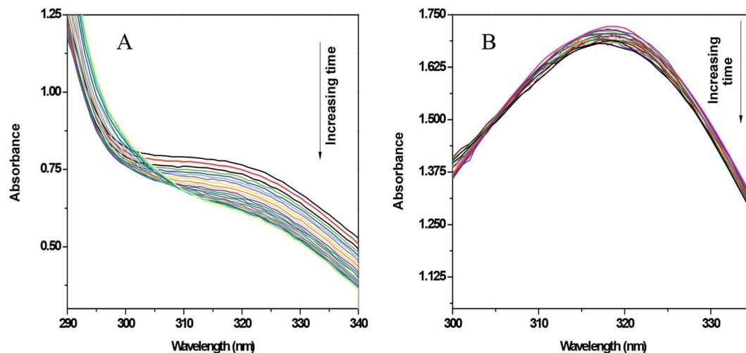
Fig. 6 UV-vis spectra of Onz (A) and Zn(Onz) 2 Cl 2 (B) in the presence of hypoxanthine in 5% DMF and xanthine oxidase. Spectra of each compound were taken at intervals of 5 minutes for 2 hours. Enzyme activity = 0.2 units per mL in XOD and compound concentration = 80 μM.
