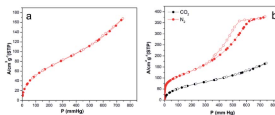
Fig. 7 Nitrogen adsorption/desorption isotherm of 3 (a), nitrogen adsorption/desorption and carbon dioxide adsorption/desorption isotherms of 5 (b).
