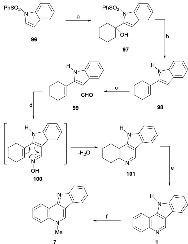
Scheme 23 Reagents and conditions: (a) LDA, THF, -78\text{ }^{\circ}\text{C} , cyclohexanone, 4 h (86%); (b) TBAF, THF, reflux, 2 h (84%); (c) \text{POCl}_3 , DMF, rt, 1 h (88%); (d) \text{NH}_2\text{OH}\cdot\text{HCl} , NaAcO, dioxane, reflux, 24 h (78%); (e) Pd/C, 1,2\text{-Cl}_2\text{C}_6\text{H}_4 , reflux, 20 h (88%); (f) (1) MeI, DMF, 80\text{ }^{\circ}\text{C} , 1 h; (2) \text{Na}_2\text{CO}_3 (85%).
