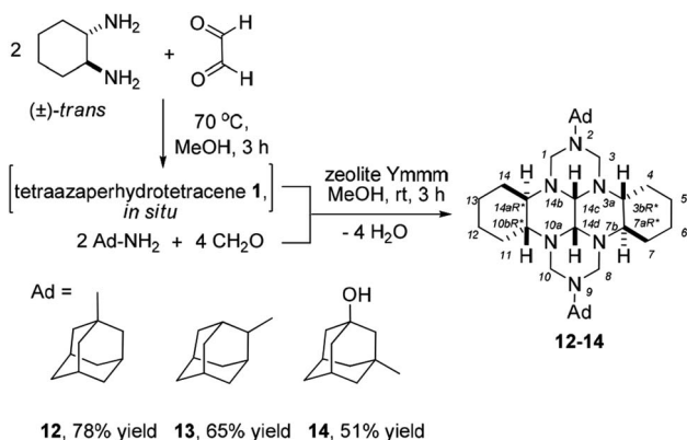
Scheme 3 Cyclocondensation reaction of adamantylamines, formaldehyde, and trans -1,6,7,12-tetraazaperhydropentacyclopentene.
