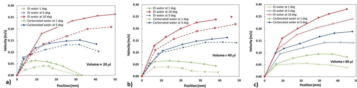
Fig. 5 The translational velocity of distilled and carbonated water droplets: (a) droplet volume is 20 μL, (b) droplet volume is 40 μL, and (c) droplet volume is 60 μL.
