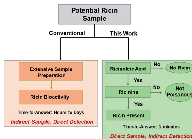
Fig. 1 Two-tiered approach to detect the presence of ricin using selected small molecule biomarkers, ricinine and ricinoleic acid, in different matrices.
