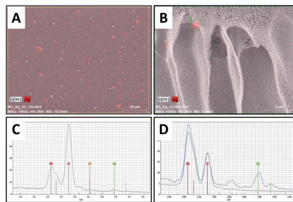
Fig. 5 SEM images of PES/PESAM/Ag composite film, (A) top surface, (B) cross section image, (C and D) EDX spectra of top and cross-sectional images, respectively.
