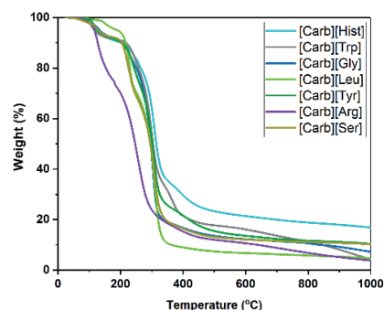
Fig. 1 Thermogravimetric analysis curves of carbohydrate/amino acid-based ILs.
