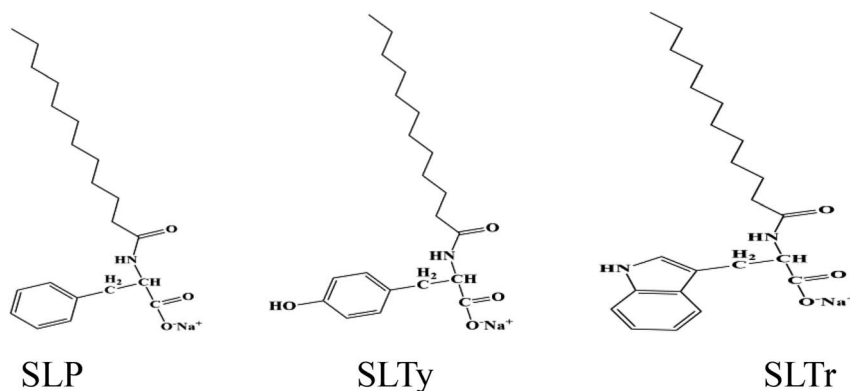
Scheme 1 Chemical structures of SLP, SLTy, and SLTr.
