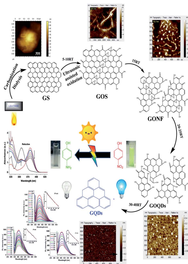
Scheme 1 Schematic synthesis of GQDs with AFM images of different stages, along with their potential catalysis, as well as sensing ability.
