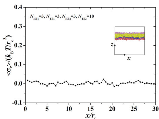
Fig. 9 The interface tension \langle \sigma_z \rangle as function of distance along x-direction for the asymmetric membrane, with N_{HB1} = 3 , N_{TB1} = 3 , N_{HB2} = 3 , and N_{TB2} = 10 . The asymmetric membranes are also inserted.
