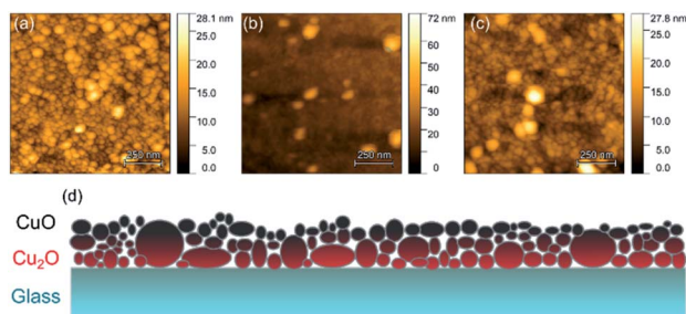
Fig. 7 (a–c) AFM images of the copper oxide samples: (a) CuO:air, (b) CuO:N, (c) CuO:O. (d) Model of the morphology and species distribution within the copper oxide films, based on the XRD, Raman, AFM, SEM and NEXAFS data.
