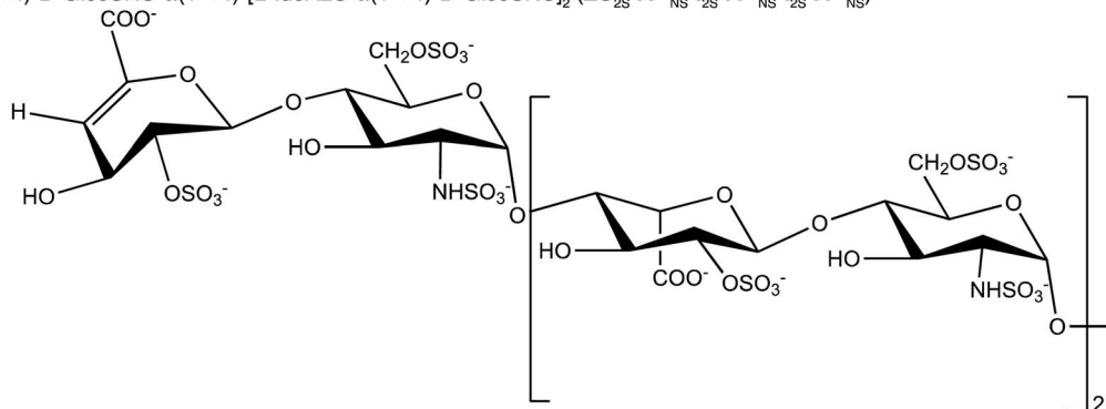
Fig. 1 Illustration of the structures of (A) heparin, the major repeating unit of which is the trisulfated disaccharide I_{2S}-A_{NS}^{6S} ; (B) the nominal reducing end of DAL , an iduronic acid group linked to 2,5 anhydrous-D-mannitol (2,5-AM-ol), the terminal group can also be sulfated at position 6 (6-O-sulfo-2,5-anhydro-D-mannitol); (C) fondaparinux ( FP ), (D) the trisulfated heparin hexasaccharide DP6 and (E) OXT , where the amino acids are labelled in blue. I stands for iduronate, G for glucuronic acid, A for glucosamine, \Delta U for an unsaturated uronic acid and nr indicates that the residue is at the nonreducing end of the molecule. The sub- and superscripts denote the position of sulfation (S) or acetylation (NAc), respectively. AN and IN refer to position N (either C atom or H atom depending on the context) of the glucosamine or iduronate residue, respectively. For example, I_{2S}-A_{NS}^{6S} corresponds to the disaccharide 2-O sulfated iduronic acid linked to 6-O-sulfated N-sulfated glucosamine. A2* signifies position 2 of glucosamine, which is N-sulfated and O-sulfated at positions 6 and 3.
