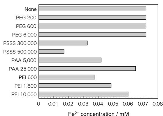
Fig. 3 Fe 2+ concentration of FeCl 2 solutions including polymers of varying molecular weight.
