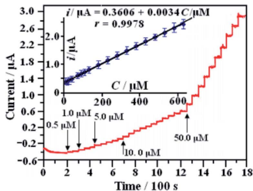
Fig. 10 i-t response of a modified electrode recorded at 0.60 V with the successive addition of amounts of glucose; the inset shows the linear relationship between i and C of glucose [reprinted with permission from ref. 97, Copyright© Elsevier].
