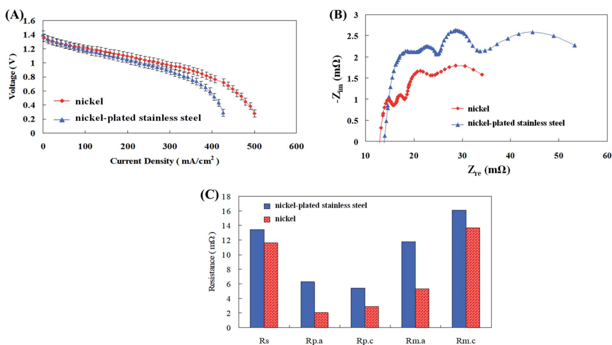
Fig. 5 (A) I - V polarization curves, (B) AC impedance spectra, and (C) impedance of fitting equivalent circuit with different anode collector plate materials.
