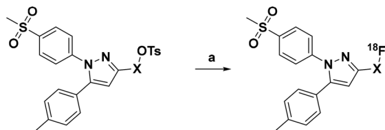
Scheme 2 Radiosynthesis of the ^{18}\text{F} -labeled celecoxib derivatives [^{18}\text{F}]\mathbf{5a,b} and [\text{D}_2, ^{18}\text{F}]\mathbf{5a} . Reagents and conditions: (a) ^{18}\text{F} fluoride/ \text{K}_2\text{CO}_3 /Kryptofix® 222 ( \text{K}_{222} ), MeCN, 80 °C, 15 min.
