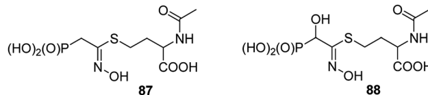
Fig. 31 Naturally occurring phosphonate peptidomimetics.
