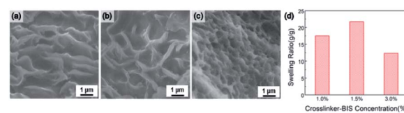
Fig. 6 SEM images of IPN-pNIPAm@Fe 2 O 3 -SiO 2 nanogels with different BIS crosslinker concentration: (a) AAm/NIPAm (30/70)-1.0%BIS, (b) AAm/NIPAm (30/70)-1.5%BIS, (c) AAm/NIPAm (30/70)-3.0%BIS, and (d) the effect of BIS crosslinker concentration on the swelling property of IPN-pNIPAm@Fe 2 O 3 -SiO 2 nanogels.
