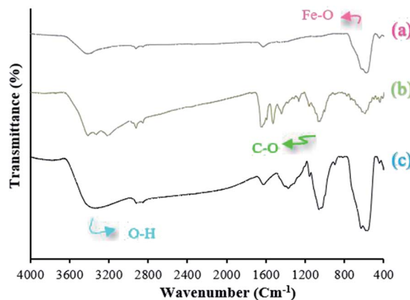
Fig. 1 FT-IR spectra of (a) \text{Fe}_3\text{O}_4 , (b) \text{Fe}_3\text{O}_4@\text{NFC} and (c) \text{Fe}_3\text{O}_4@\text{NFC}@\text{Co(II)} .
