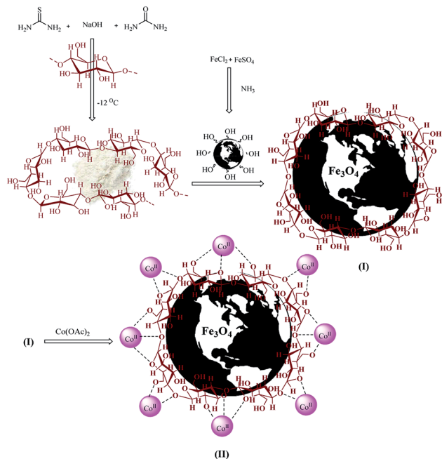
Scheme 1 The synthetic route for \text{Fe}_3\text{O}_4@\text{NFC}@\text{Co(II)} .
