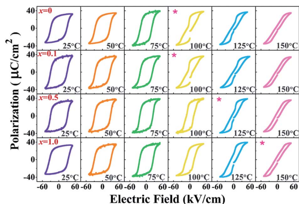
Fig. 7 Temperature dependence on polarization–electric field ( P – E ) hysteresis loops of the BNT–6BT/ x\text{Al}_2\text{O}_3 ceramics where x = 0 –1.0 mol%, measured under an electric field of 50 kV \text{cm}^{-1} and a frequency of 1 Hz.
