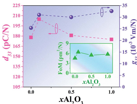
Fig. 10 Plots of low-field piezoelectric coefficients ( d_{33} ) and piezoelectric voltage coefficient ( g_{33} ) as a function of \text{Al}_2\text{O}_3 content of the BNT–6BT/ x\text{Al}_2\text{O}_3 ceramics (the inset shows: FoM as a function of \text{Al}_2\text{O}_3 content).
