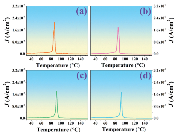
Fig. 5 Plots of current density–temperature ( J - T ) from the TSDC technique of the BNT-6BT/ x\text{Al}_2\text{O}_3 ceramics.
